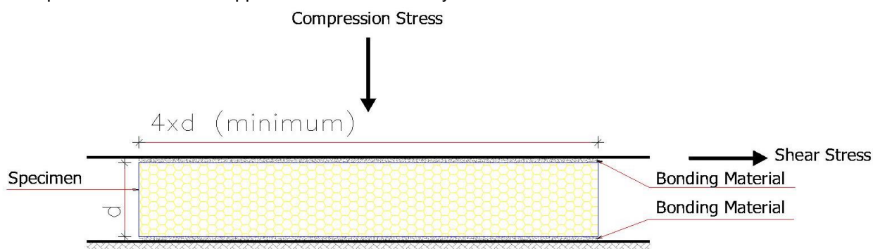
Figure (2) – Sketch of the Combined Shear-Compression Creep Test-Setup
