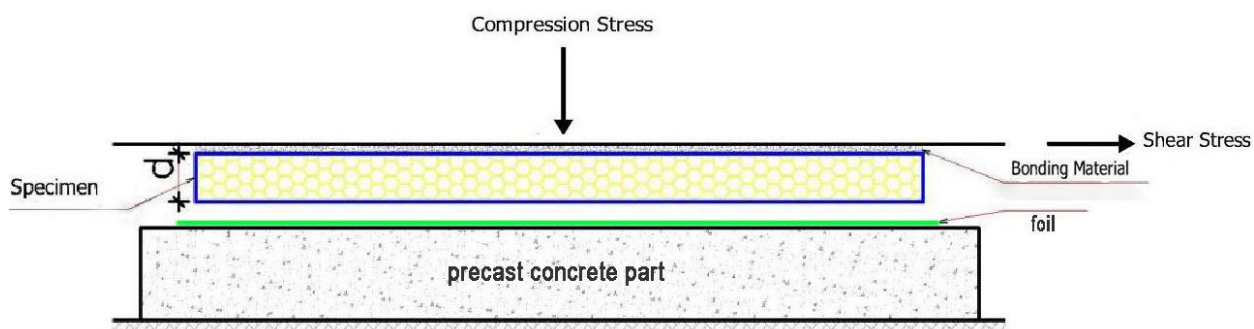
Figure (4) – Sketch of the test-setup to determine the adhesive friction coefficient between the expanded polystyrene foam boards and a concrete finished part with foil
