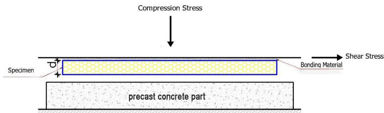
Figure (6) – Sketch of the test-setup to determine the adhesive friction coefficient between the expanded polystyrene foam boards and a concrete finished part without foil
