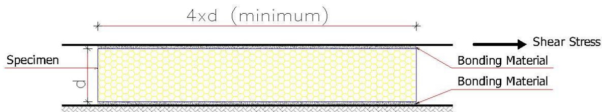
Figure (1) – Sketch of the Shear Creep Test-Setup
