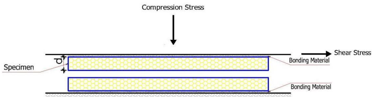
Figure (3) – Sketch of the test-setup to determine the adhesive friction coefficient between the expanded polystyrene foam boards
