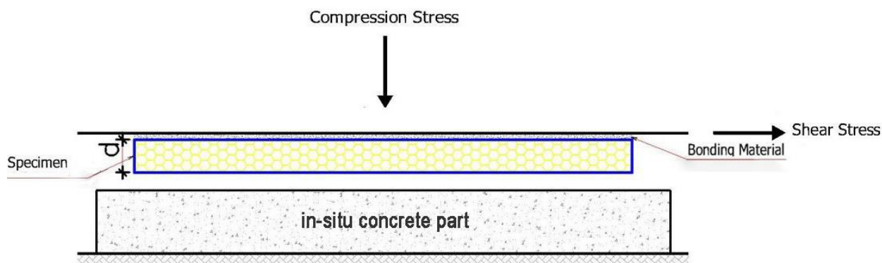
Figure (5) – Sketch of the test-setup to determine the adhesive friction coefficient between the expanded polystyrene foam boards and a concrete finished part without foil
